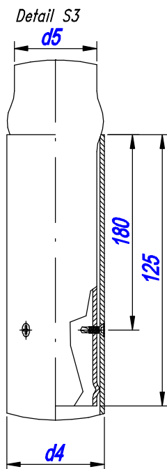
Base compartment Aukko
